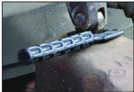
PIN LIFTER WRENCH (Coupler END) SECO-PLT-1
