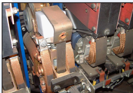
CONTACTOR GUARD SECO-SCG-22
