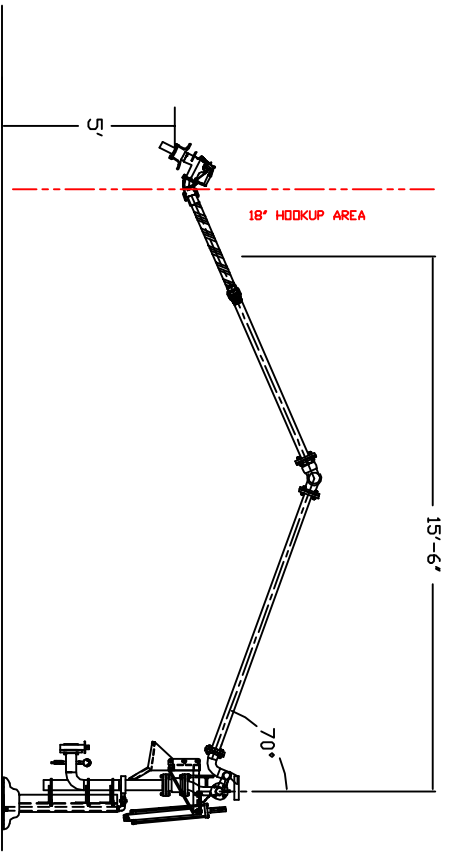
104-HP-1 GODDSNECK STYLE FUELCRANE
