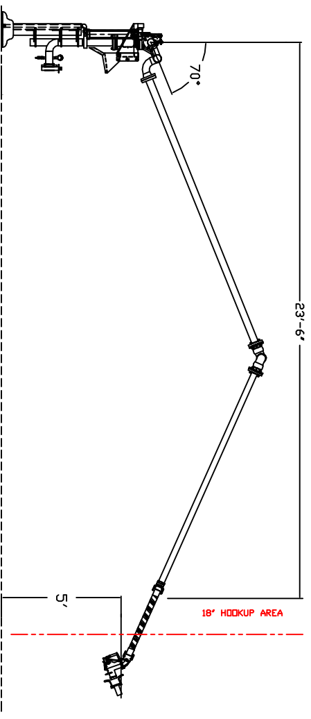
104-HP-2 GODDSNECK STYLE FUELCRANE
